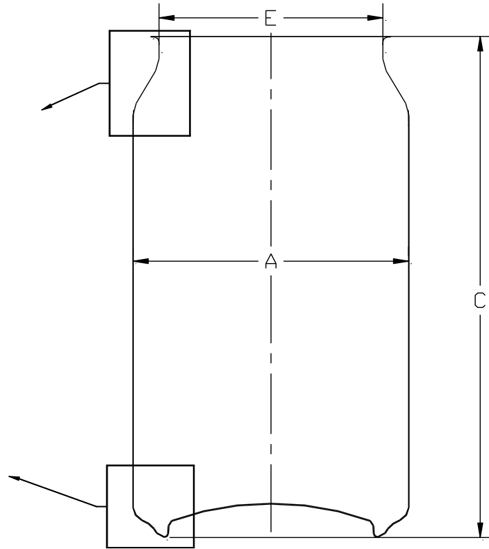
NECKED & FLANGED CAN
